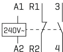
240V Coil 1 NO + 1NC contact
