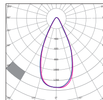
50 Degree Lens
