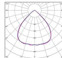
90 Degree Lens
