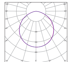
120 Degree Lens
