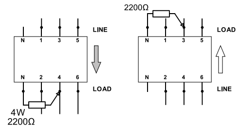
3 Phase Connection without Neutral 380-415V
