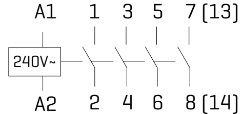
240V Coil 4 NO contacts
