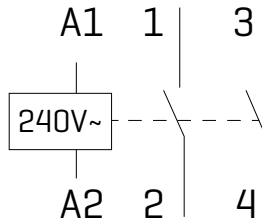
240V Coil 2 NO contacts
