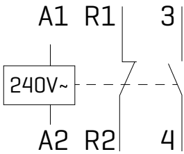
240V Coil 1 NO + 1NC contact
