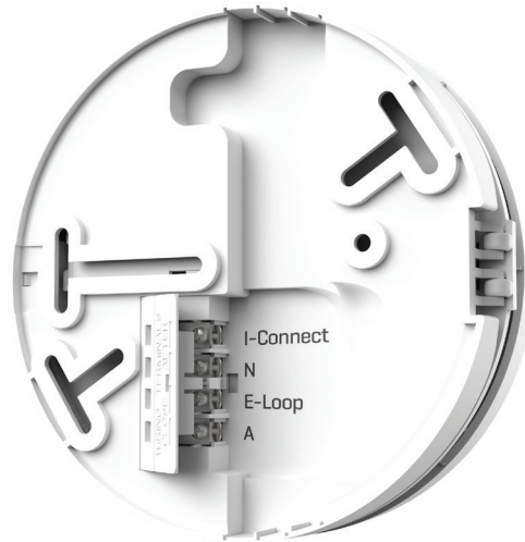
Back Side
