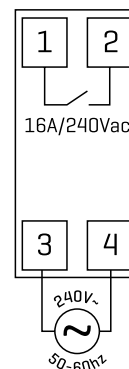
Wiring Diagram
