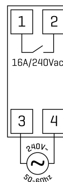
Wiring Diagram
