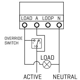
Installation with override
