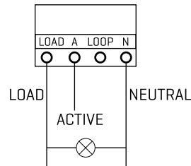
Basic installation
